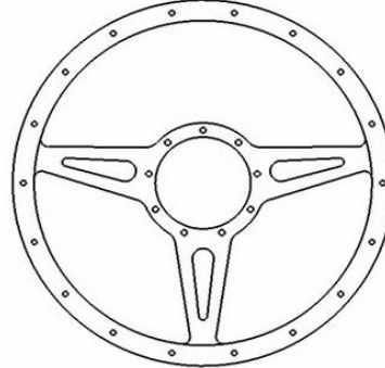
Classic 3 14" diameter (355 mm) Big Slots Flat or Dished
