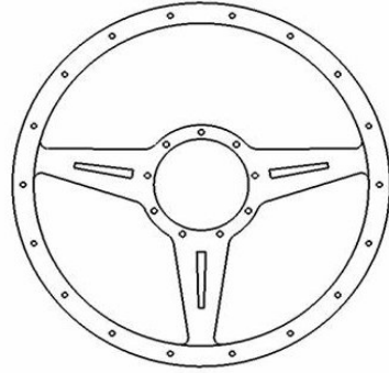
Classic 3 14" diameter (355 mm) Little Slots Flat or Dished
