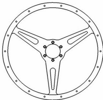
Derrington Style 15" diameter (380 mm) Big Slots Flat or Dished
