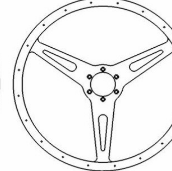
Derrington Style 16" diameter (405 mm) Big Slots Flat or Dished
